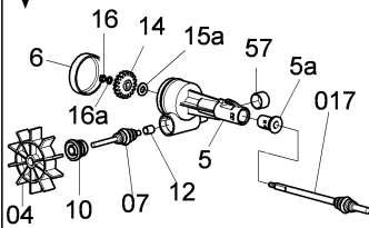
Pos.05 - Cod.10432
