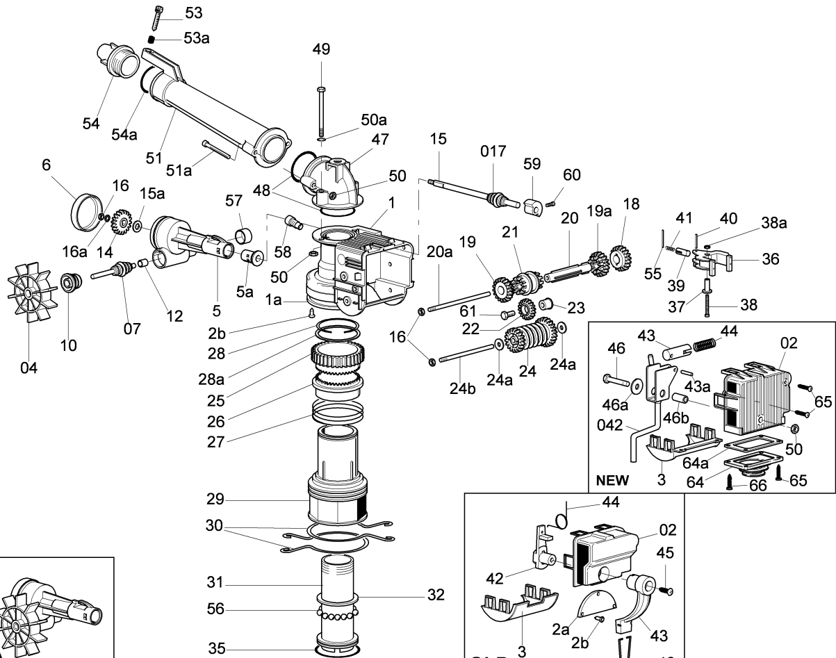
Pos.05 - Cod.10432
